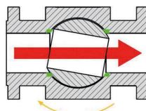
2° stage PST operation (PST set point achieved) 10% rotation
